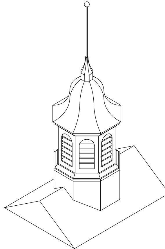
Isometric View:
